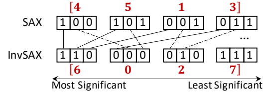
Figure 5: SEAsam transformation and InvSAX [23].
