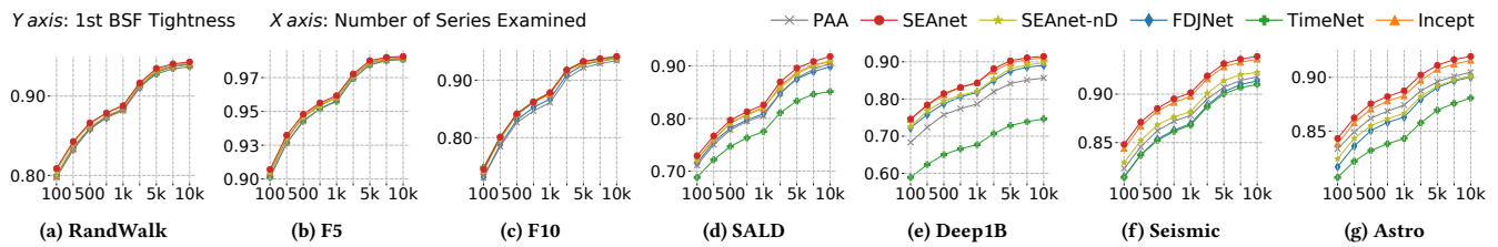
Figure 8: Approximate query answers quality: 1st BSF tightness vs number of series visited; 100M series datasets (higher is better)
