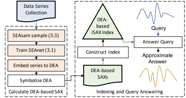
Figure 3: Workflow of DEA-based approximate similarity search.
