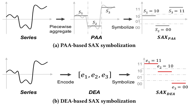
Figure 2: Replace PAA by DEA for SAX symbolization.
