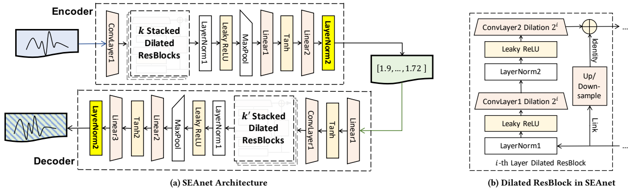
Figure 4: The SEAnet architecture and the details of a dilated full-preactivation ResBlock.
