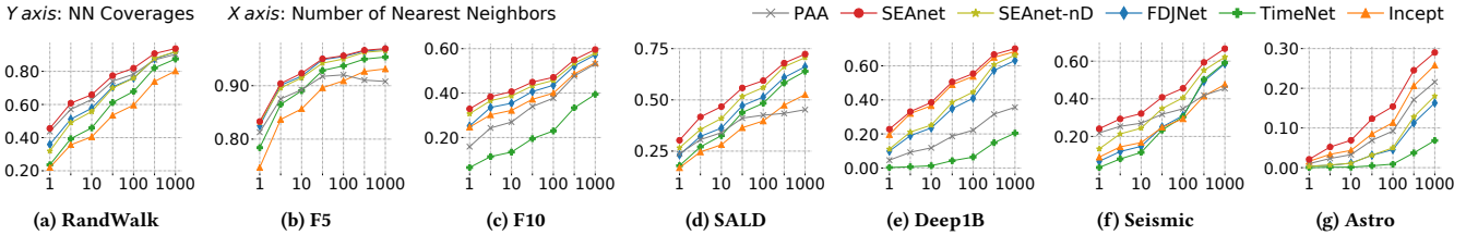
Figure 7: Nearest neighbors' coverage vs neighborhood size (higher is better).
