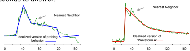
Figure 10. Query time series, and its approximate nearest neighbor.
