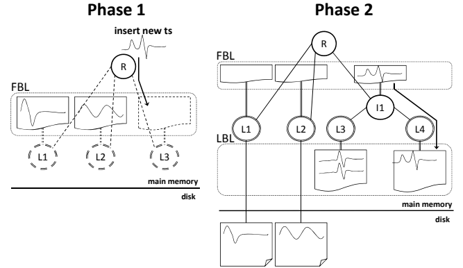
Figure 2. The bulk loading algorithm. left ) Phase 1 fills the FBL buffers with time series until main memory is full. right ) Phase 2, processing subtree rooted at node I1 (subtrees rooted at nodes L1 and L2 have already been flushed to disk).
