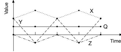
Figure 1: Euclidean distance fails to distinguish between the X and Y series, given query Q .
