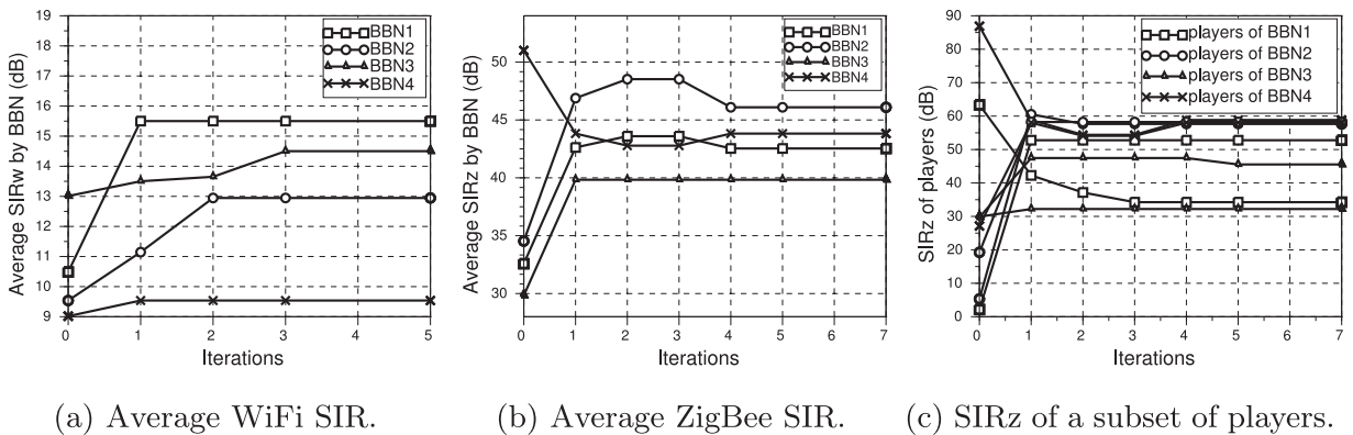
Fig. 9. Dynamics of the BR-SIM algorithm for each BBN, with N = 40 WBANs.
