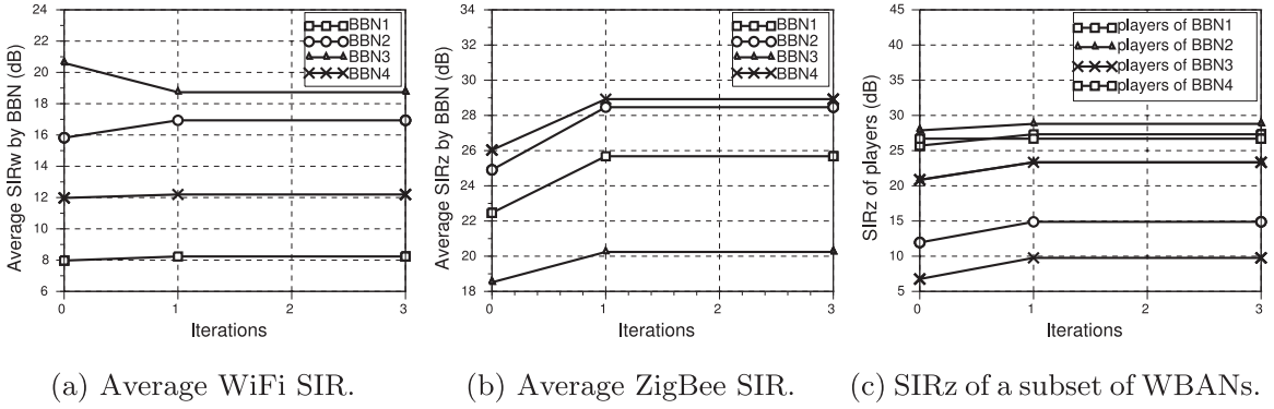
Fig. 14. Dynamics of the PAPU algorithm for each BBN, with N = 40 WBANs.
