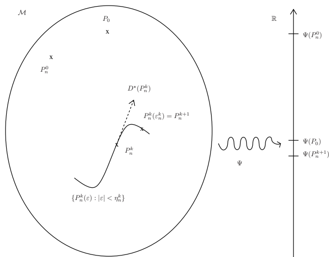
FIG 1. Illustration of the TMLE procedure (with its general one-step updating procedure). We intentionally represent the initial estimator P_n^0 closer to P_0 than its k th and (k+1) th updates P_n^k and P_n^{k+1} , heuristically because P_n^0 is as close to P_0 as one can possibly get (given P_n and the specifics of the super-learning procedure) when targeting P_0 itself. However, this obviously does not necessarily imply that \Psi(P_n^0) performs well when targeting \Psi(P_0) (instead of P_0 ), which is why we also intentionally represent \Psi(P_n^{k+1}) closer to \Psi(P_0) than \Psi(P_n^0) . Indeed, P_n^{k+1} is obtained by fluctuating its predecessor P_n^k “in the direction of \Psi ”, i.e., taking into account the fact that we are ultimately interested in estimating \Psi(P_0) . More specifically, the fluctuation \{P_n^k(\varepsilon) : |\varepsilon| < \eta_n^k\} of P_n^k is a one-dimensional parametric model (hence its curvy shape in the large model \mathcal{M} ) such that (i) P_n^k(0) = P_n^k , and (b) its score at \varepsilon = 0 equals the efficient influence curve D^*(P_n^k) at P_n^k (hence the dotted arrow). An optimal stretch \varepsilon_n^k is determined (e.g. by maximizing the likelihood on the fluctuation), yielding the update P_n^{k+1} = P_n^k(\varepsilon_n^k) .
