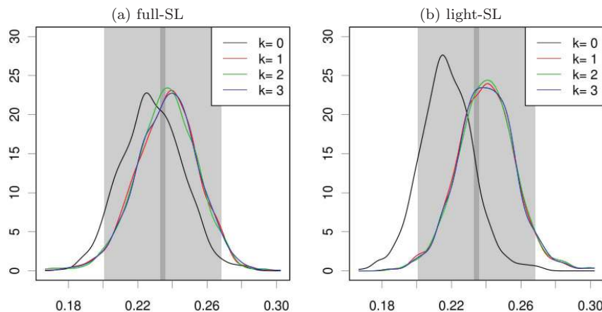
FIG 3. Empirical distribution of \{\psi_{n,b}^k : b \leq B'\} based on n = 200 independent observed data structures for k = 0 (initial estimator) and k iterations of the updating procedure ( k = 1, 2, 3 ), as obtained from B' = 10^3 independent replications of the simulation study (using a Gaussian kernel density estimator). (a). The super-learning procedure involves all algorithms described in Section 6.5. (b). The super-learning procedure only involves algorithms based on generalized linear models. In both graphics, gray rectangles represent 95%-accuracy intervals [\psi_B(P^s) \pm \xi_{0.975} \sqrt{v_B(P^s)/n}] and [\psi_B(P^s) \pm \xi_{0.975} \sqrt{v_B(P^s)/B}] for the true parameter \Psi(P^s) based on 200 observed data structures (light gray) and B = 10^5 observed data structures (dark gray). The length of [\psi_B(P^s) \pm \xi_{0.975} \sqrt{v_B(P^s)/n}] is the optimal length of a 95%-confidence interval based on an efficient (regular) estimator of \Psi(P^s) relying on n observations (assuming that the asymptotic regime is reached).
