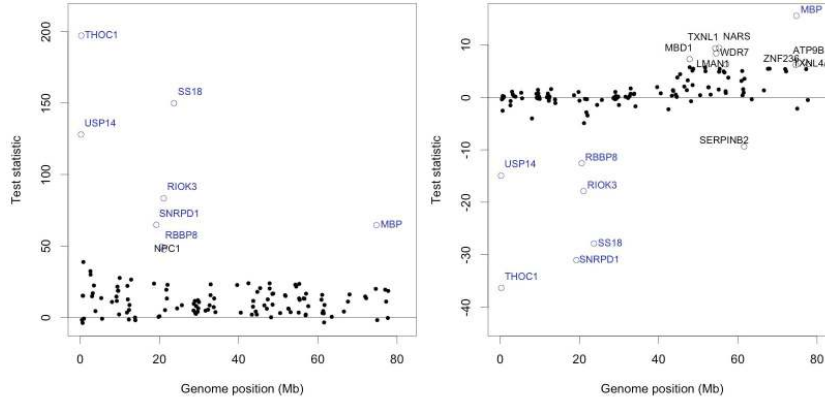
FIG 4. Real data application to the 130 genes of chromosome 18 in the OvCa dataset (ovarian cancers). We represent the test statistics \sqrt{n}(\psi_n^{g,3} - \psi_{\text{ref}}^g)/s_n^{g,3} for \psi_{\text{ref}}^g = 0 (left graphic) and \psi_{\text{ref}}^g = \mathcal{F}(P_n^g) (right graphic) along the position of gene g on the genome. We report the names of the genes such that \sqrt{n}|\psi_n^{g,3}|/s_n^{g,3} > 45 (left graphic) and \sqrt{n}|\psi_n^{g,3} - \mathcal{F}(P_n^g)|/s_n^{g,3} > 6 (right graphic), the cut-offs being arbitrarily chosen.
