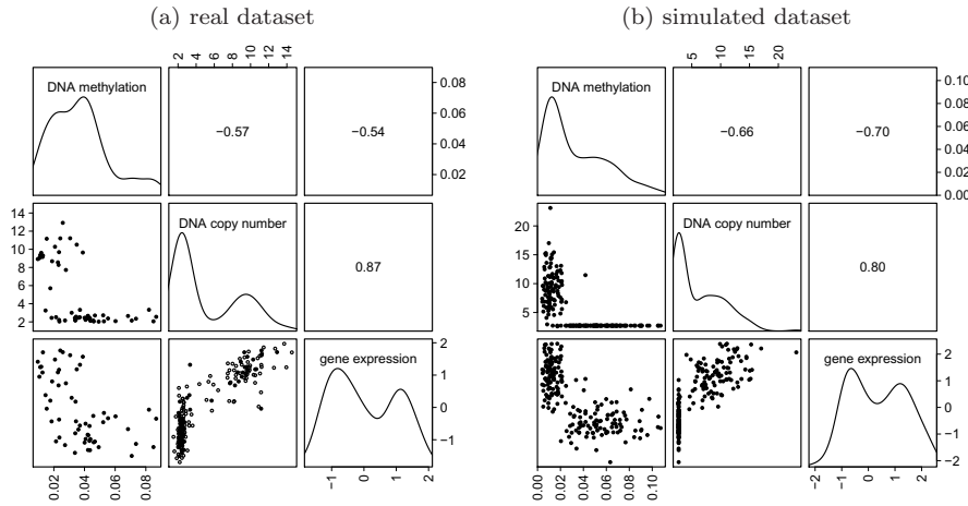
FIG 2. Illustrating DNA methylation, DNA copy number, and gene expression data. In both graphics, we represent kernel density estimates (diagonal panels), pairwise plots (lower panels), and report the pairwise Pearson correlation coefficients (upper panels). (a). Real dataset corresponding to the EGFR gene in 187 GBM tumor samples. For 130 among the 187 samples, only DNA copy number and gene expression data were available (circles in lower middle plot). (b). Simulated dataset consisting of n = 200 independent copies of the synthetic observed data structure described in Section 6.6. Note that the constant O_2^X is added to each value of X so that graphics corresponding to real and simulated data can be more easily compared.
